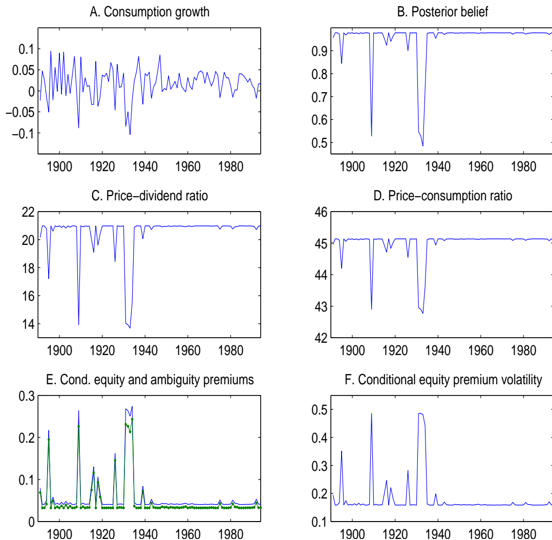
Figure 3: Implied time series of some financial variables using historical consumption growth data. This figure plots consumption growth, Bayesian posterior probabilities of the high-growth state, price-dividend and price-consumption ratios, conditional equity and ambiguity premiums, and conditional equity premium volatility. In Panel E, the solid and dotted solid lines represent conditional equity and ambiguity premiums, respectively. We take baseline parameter values calibrated in Section 4.1.
