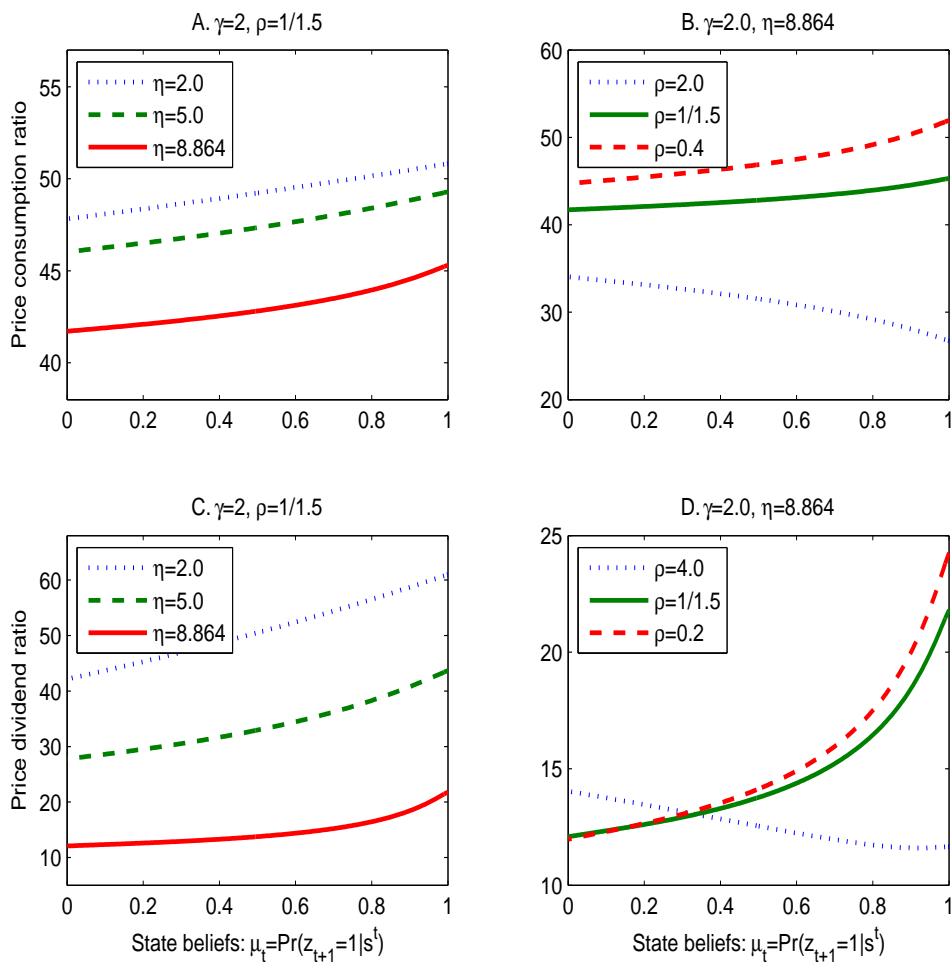
Figure 1: The price-dividend ratio and the price-consumption ratio. Panels A and B plot the price-consumption ratio of the consumption claim as a function of the Bayesian posterior probabilities of the high-growth state. Panels C and D plot the price-dividend ratio of the dividend claim as a function of the posterior probabilities of the high-growth state. We set \beta = 0.975 . The case with \gamma = \eta corresponds to the Epstein-Zin model with Bayesian learning.
