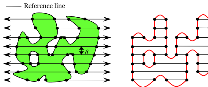
Fig. 5. Zigzag machining graph. Left: Zigzag lines intersect pocket contour; Right: corresponding machining graph
