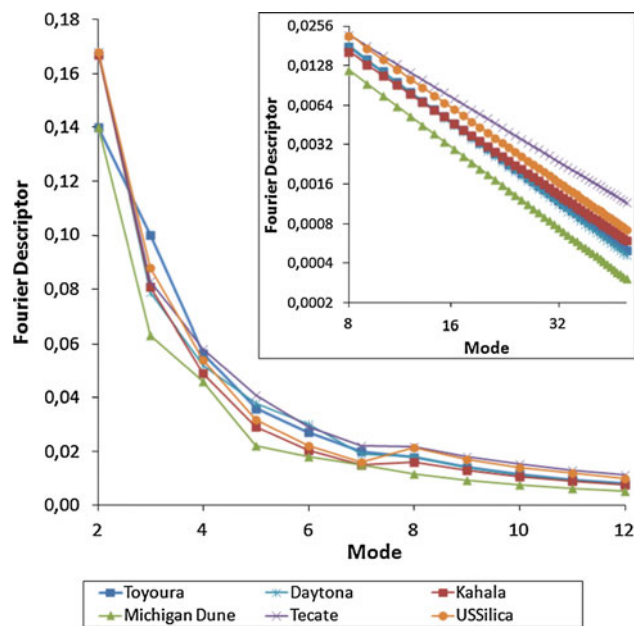
Fig. 7 Fourier spectra provided by [33] for six sands; Inset : log 2 -log 2 chart of the spectra tails
