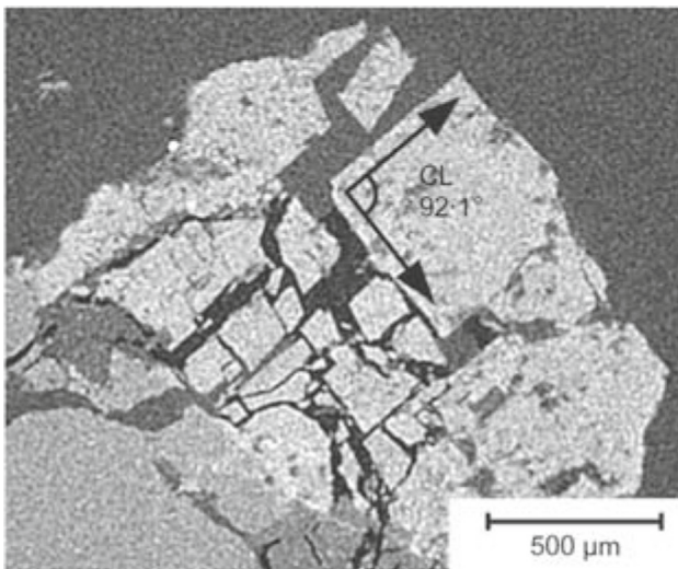
Fig. 1 Fracture pattern of a granite sand particle [1]. Cracks at right angles following the cleavage of feldspar are observed
